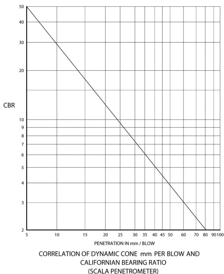
Figure 3.1 – Parameter relationship
