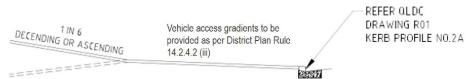
SECTION X-X
