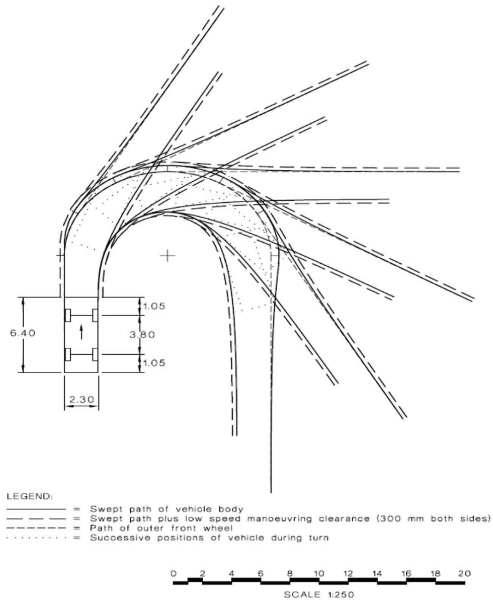
Turning Path Template - Small Rigid Vehicle Minimum Radius Turn (7.1m)
