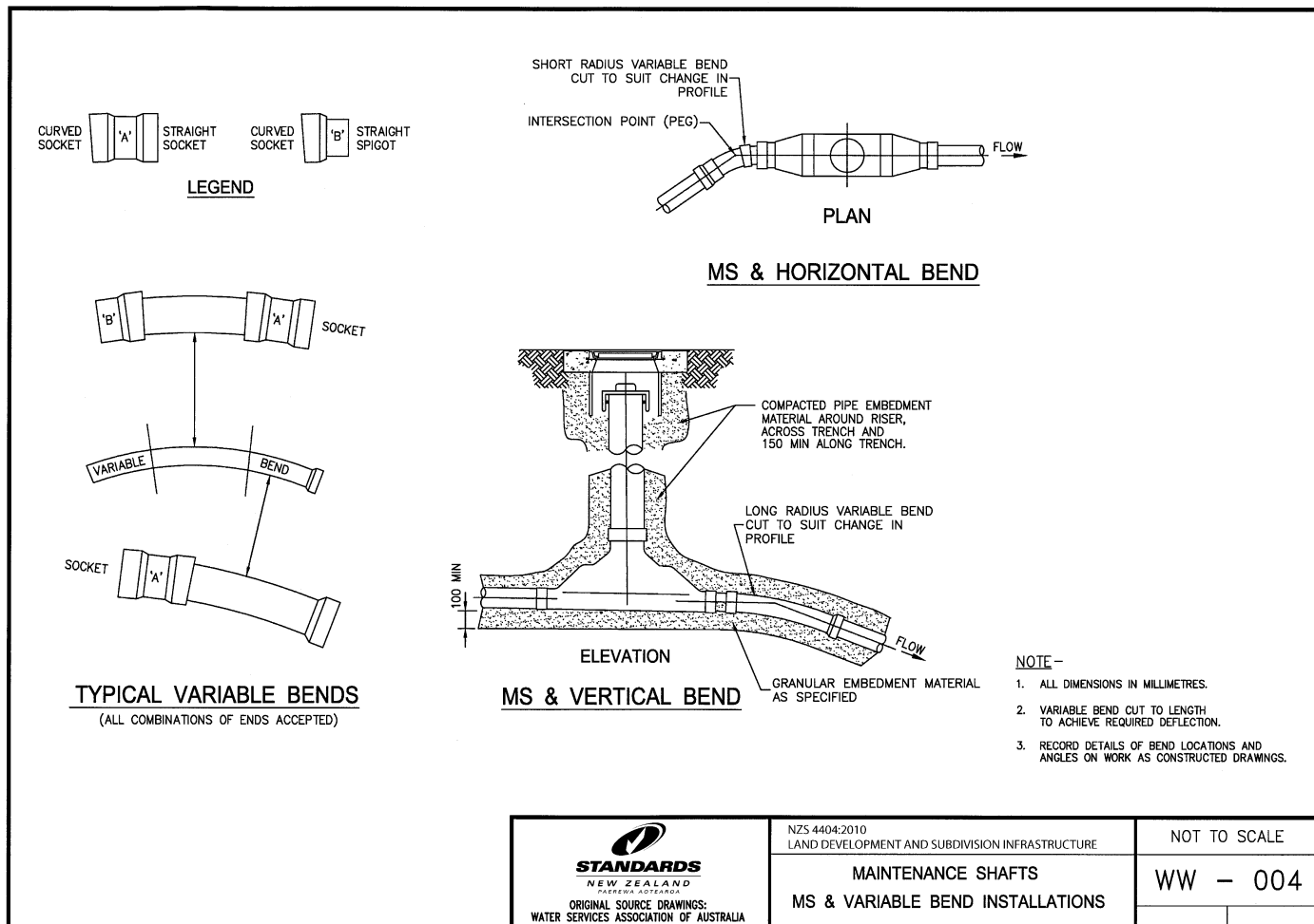
WW - 004 Maintenance shafts – MS and variable bend installations
