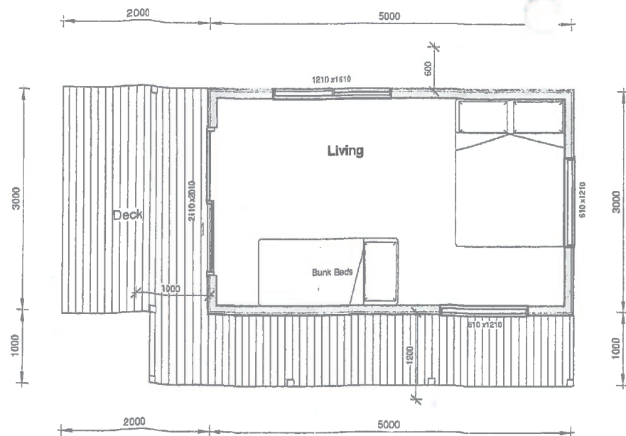
1 Floor Plan 1 : 50 Living Area 15.00 m 2
