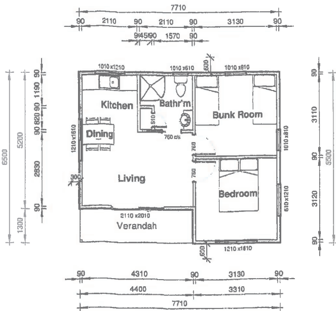
1 Floor Plan 1 : 100 Living Area 44.40 m 2
