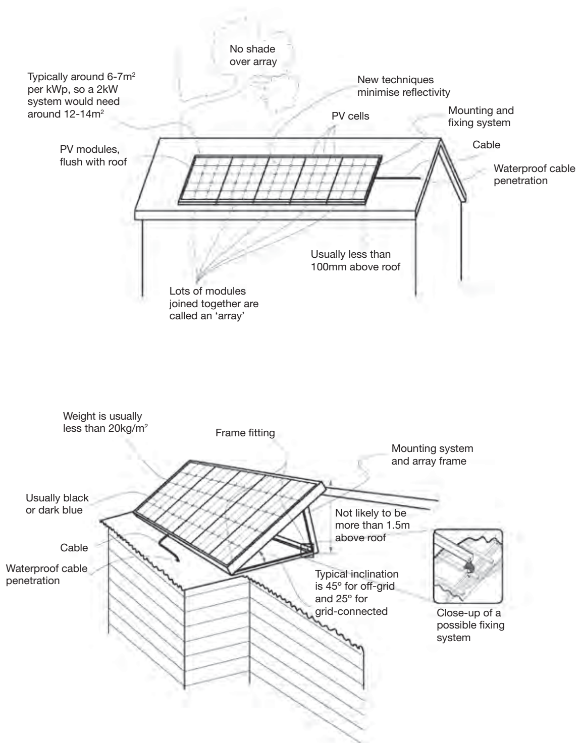
Figure 22. PV arrays, modules and cells
