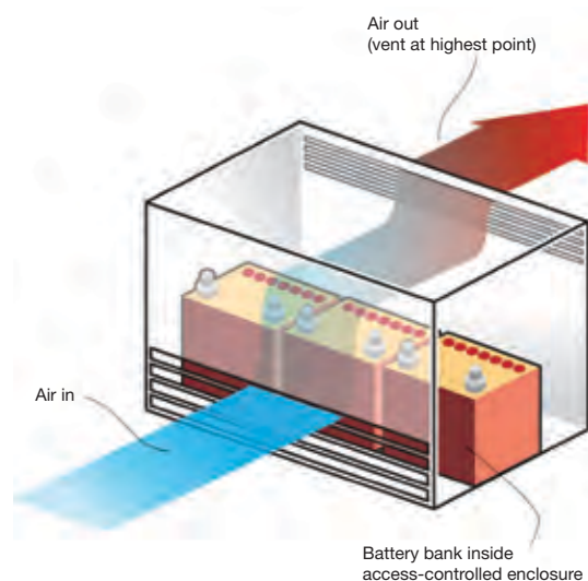
Figure 58. A typical ventilation arrangement
