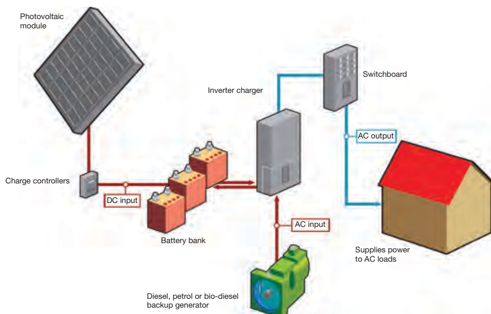
Figure 10. Example component diagram for a SAPS
