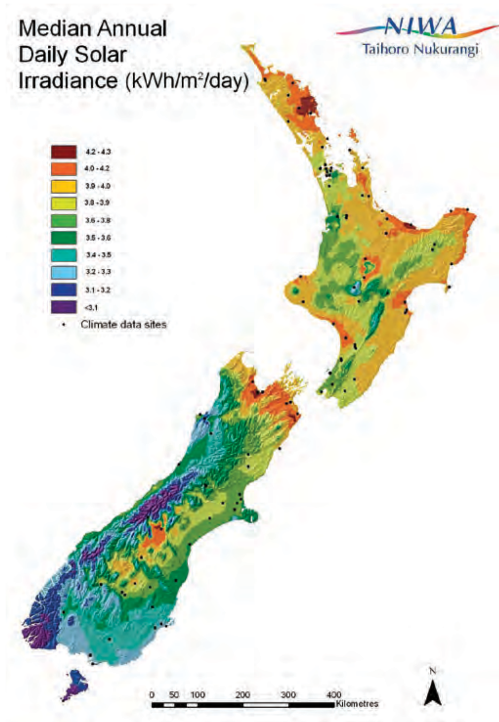
Figure 23. Map of the solar resource (kWh/m 2 /day) in New Zealand Source: NIWA (modified)
