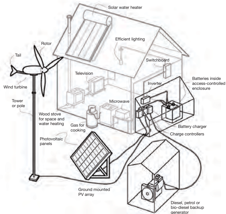
Figure 8. Main components of a SAPS
