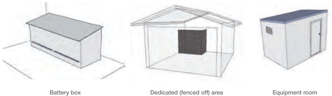
Figure 59. Some options for battery enclosures Credit: Southern Perspectives Ltd
