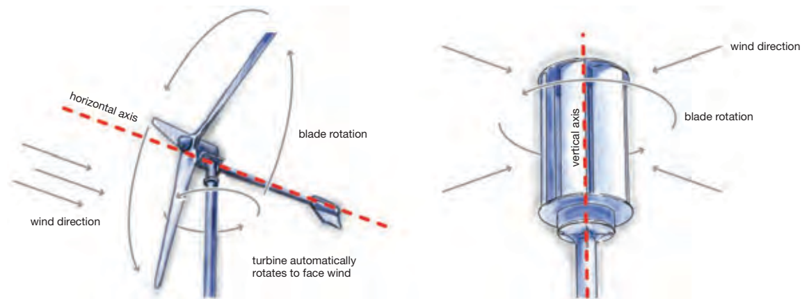
Figure 30. Illustration of horizontal (left) and vertical-axis wind turbines
