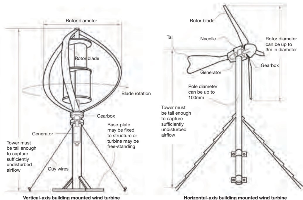
Figure 44. Examples of roof-mounted wind turbines
