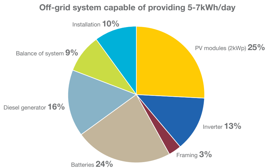
Figure 28. Indicative cost breakdown of a SAPS capable of generating between 5-7kWh/day
