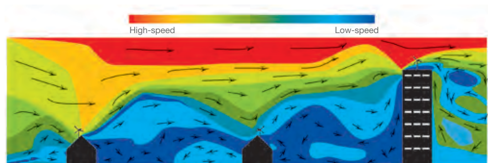
Illustration of wind-flow speeds in an urban environment. It can be more difficult to site a turbine in consistent and strong winds.
