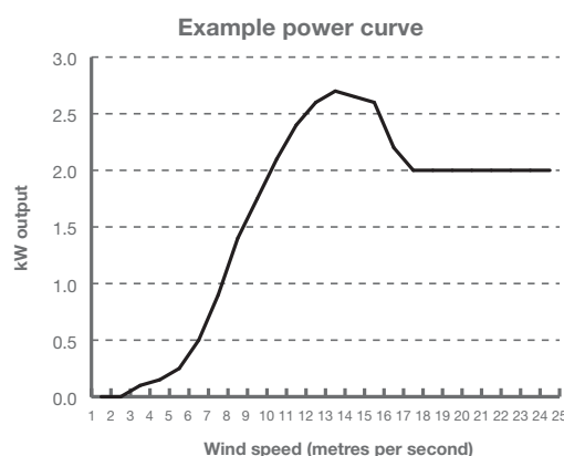
Figure 37. Example of a power curve for a small wind turbine
