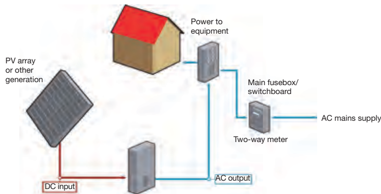
Figure 14. Example component diagram for a grid-connected system
