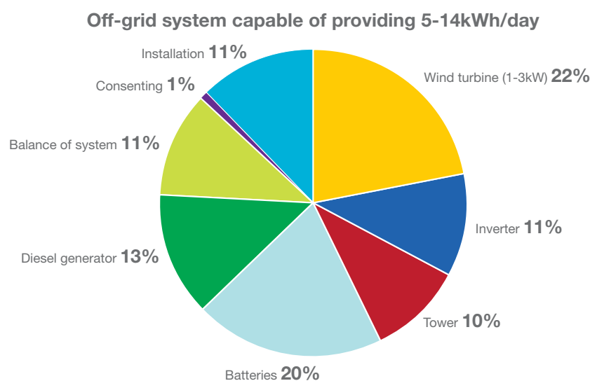
Figure 47. Indicative cost breakdown of a micro wind turbine in a stand-alone system
