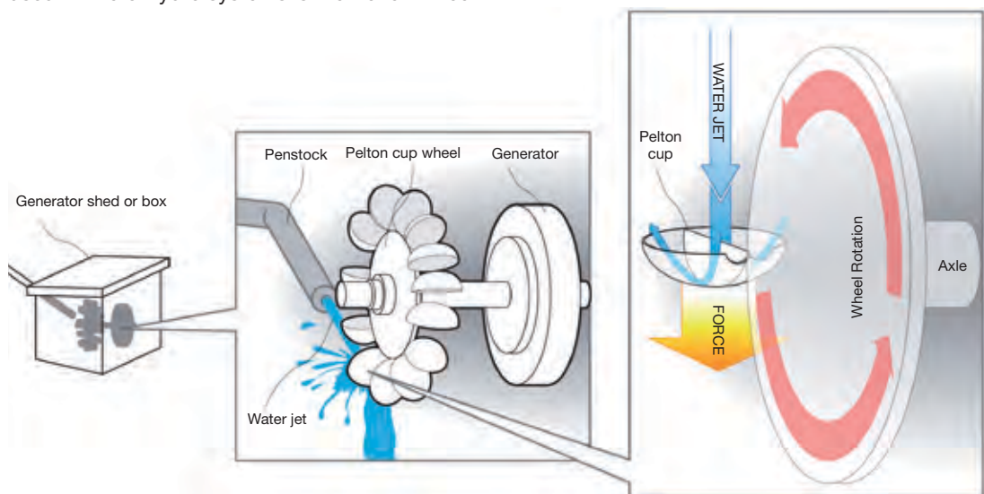
Figure 54. Example of a Pelton wheel, a form of impulse turbine
