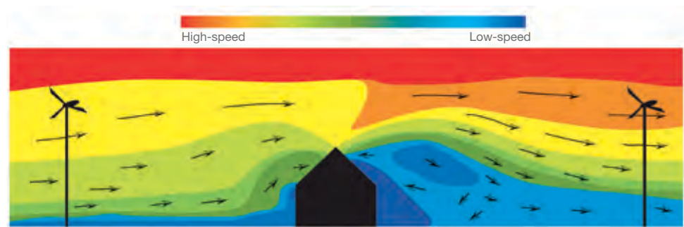
Pole-mounted turbines should be located away from obstructions such as buildings or trees. Taller poles or tower are required to position turbines in stronger and more consistent winds.
