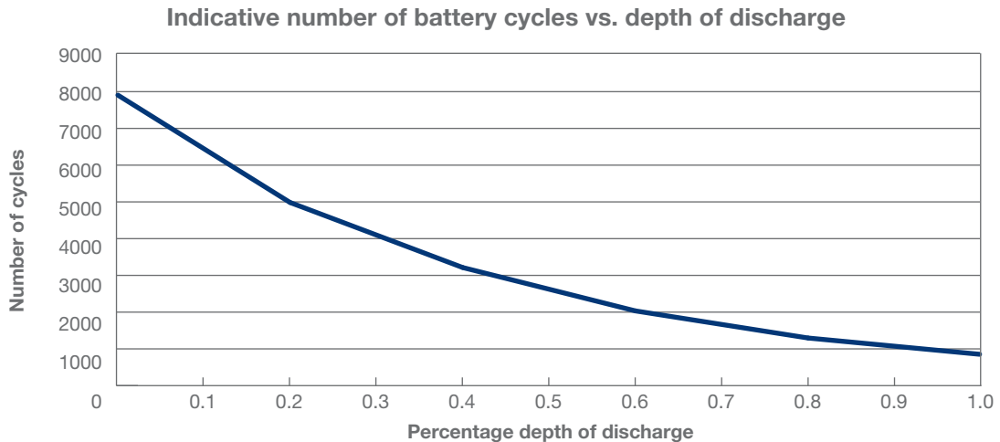
Figure 57. Battery cycle life vs. depth of discharge
