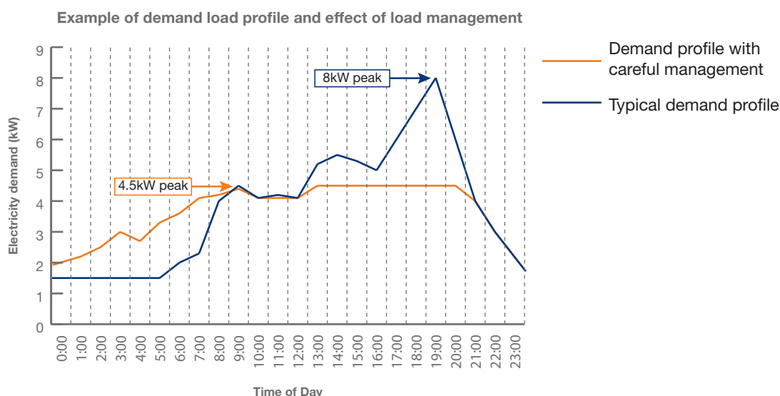
Figure 9. Load profile and example of load management
