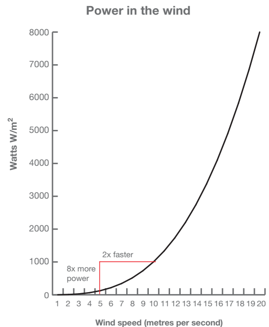
Figure 33. Power available in the wind
