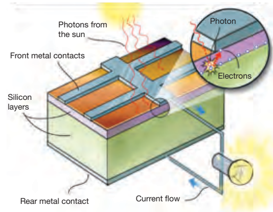
Figure 18. Cross section of a PV cell
